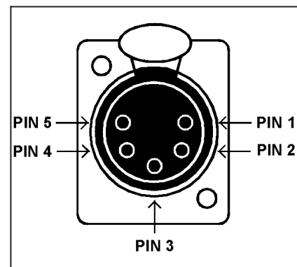
Figure 6 - 6: DMX Connector
