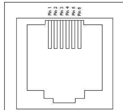
Figure 6 - 7: RJ12 Connector
