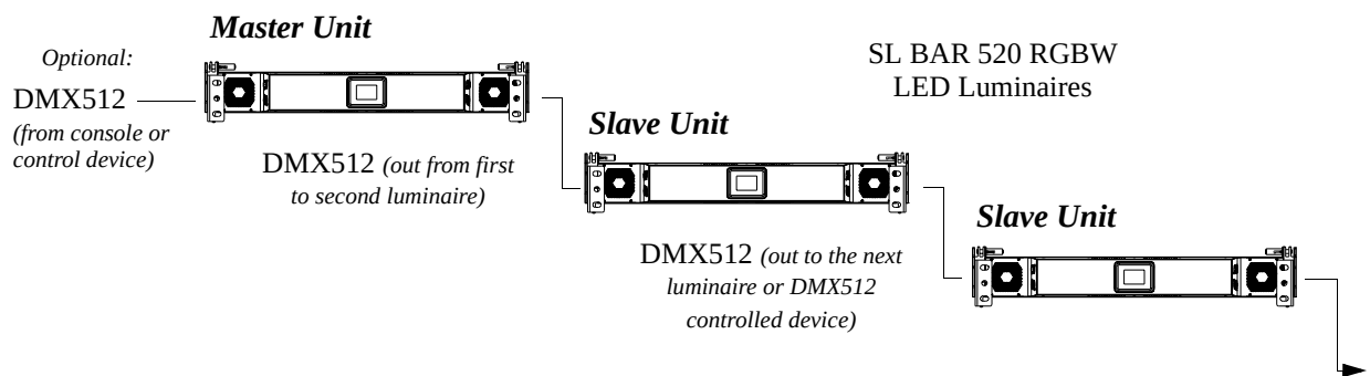
Figure 15: SL BAR 520 RGBW LED Luminaire - Master / Slave Configuration
