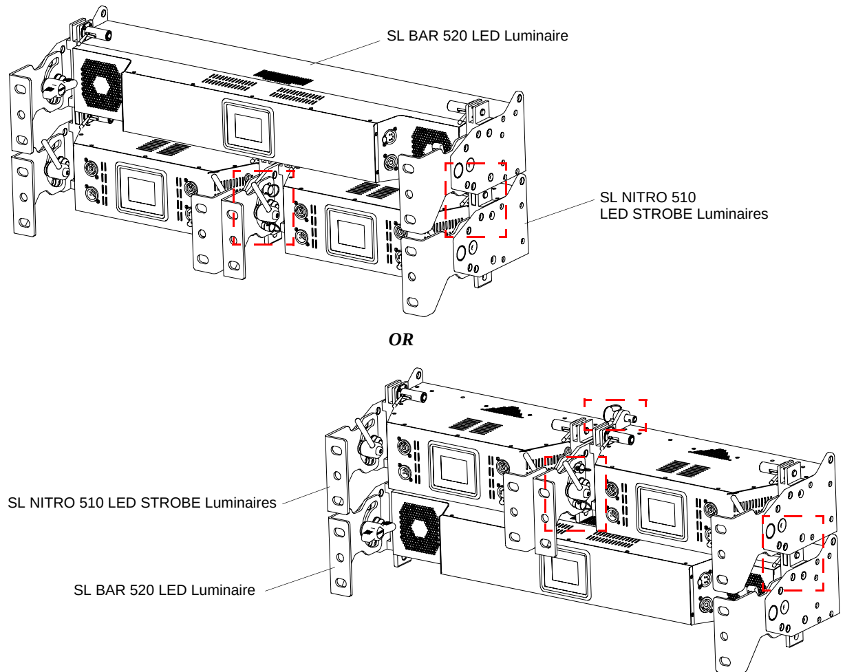
Figure 11: SL BAR 520 RGBW LED Luminaires - Connections
