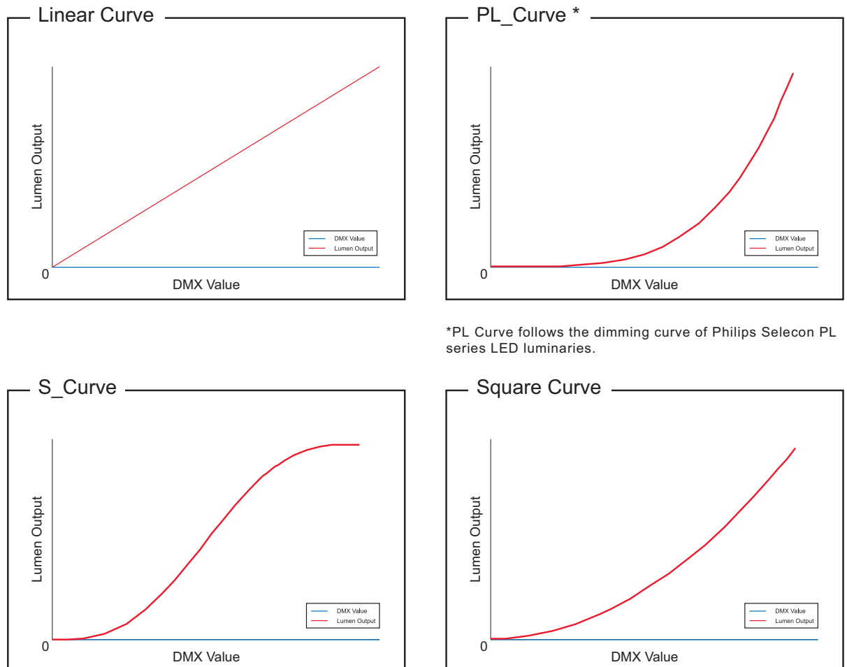
Figure 14: SL BAR 520 RGBW LED Luminaire Dimmer Curves
