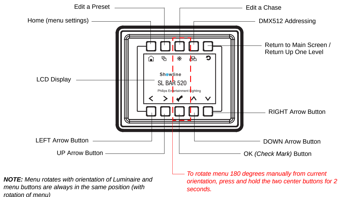
Figure 13: LCD Display and Menu System
