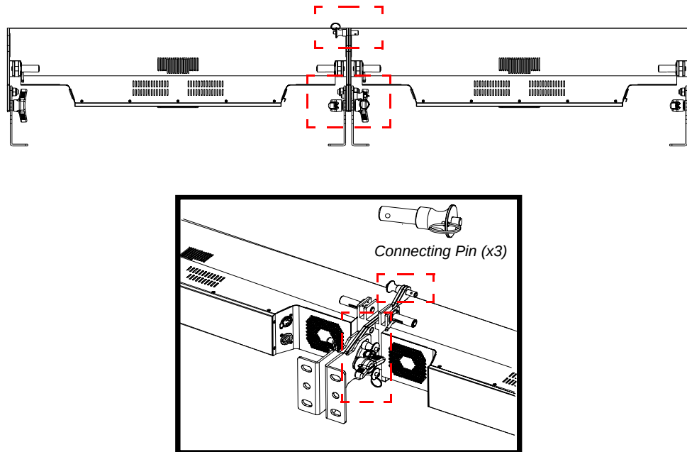
Figure 9: Connecting Luminaires Side-to-Side
