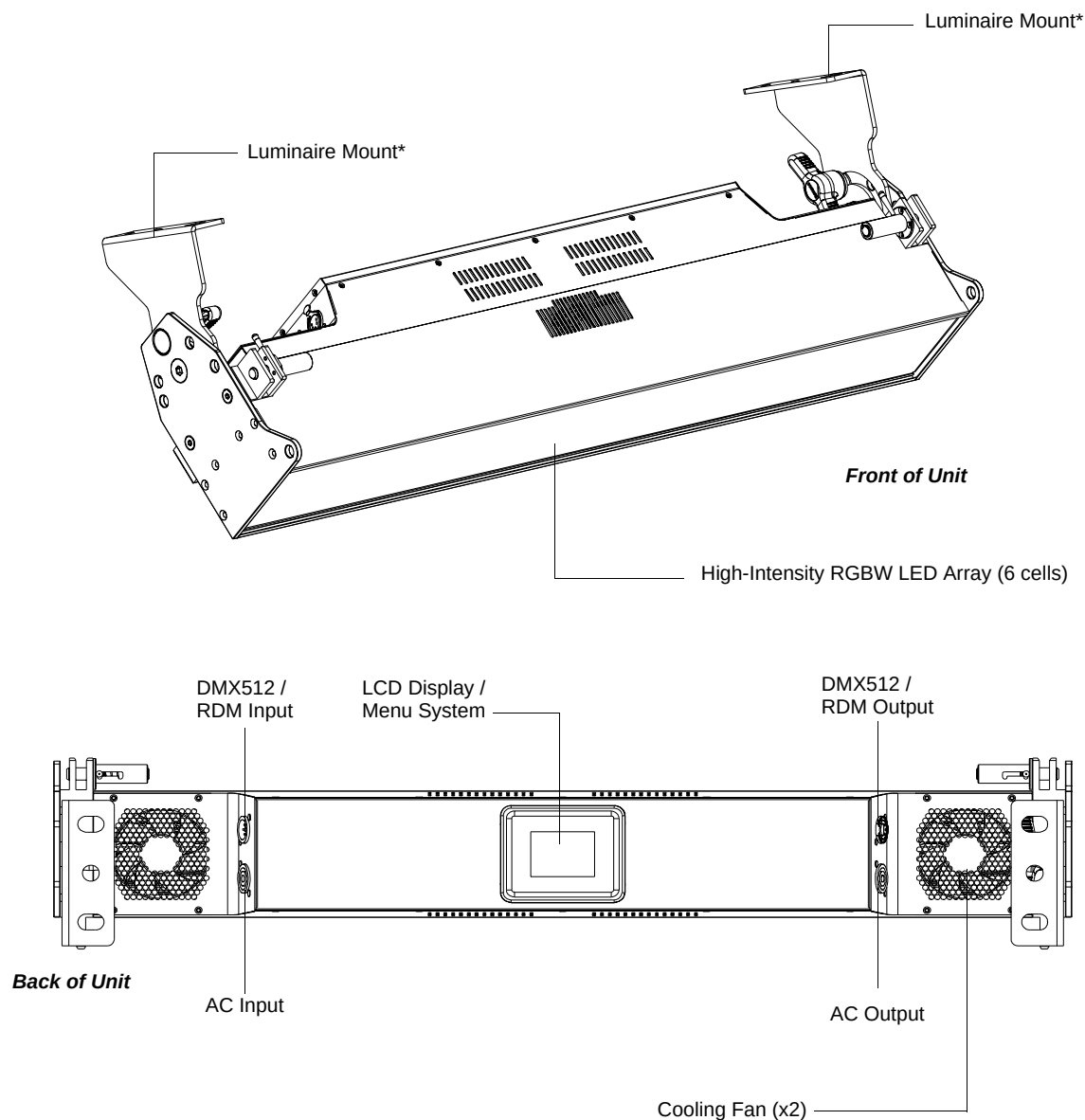
Figure 2: SL BAR 520 RGBW LED Luminaire Components
