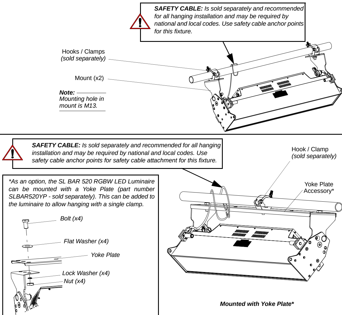
Figure 7: Mounting Luminaire - Hanging Applications
