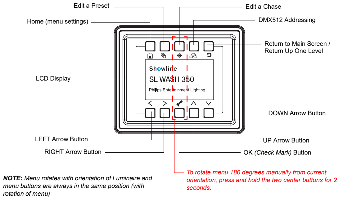
Figure 8: LCD Display and Menu System
