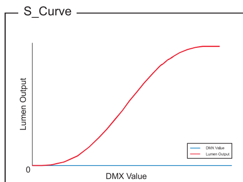
Figure 9: SL WASH 350 RGBW LED Luminaire Dimmer Curves
