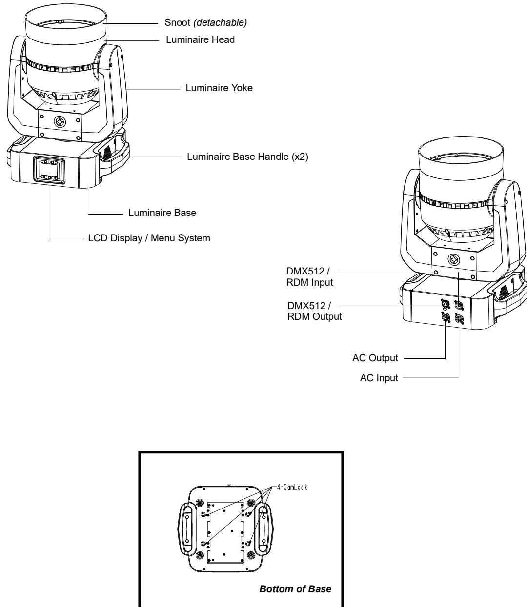
Figure 2: SL WASH 350 RGBW LED Luminaire Components
