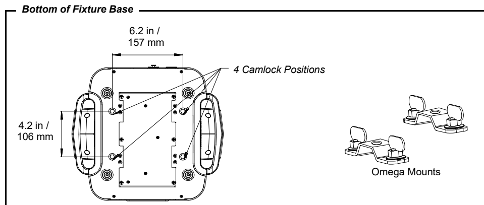
Figure 7: Mounting Luminaire - Hanging Applications
