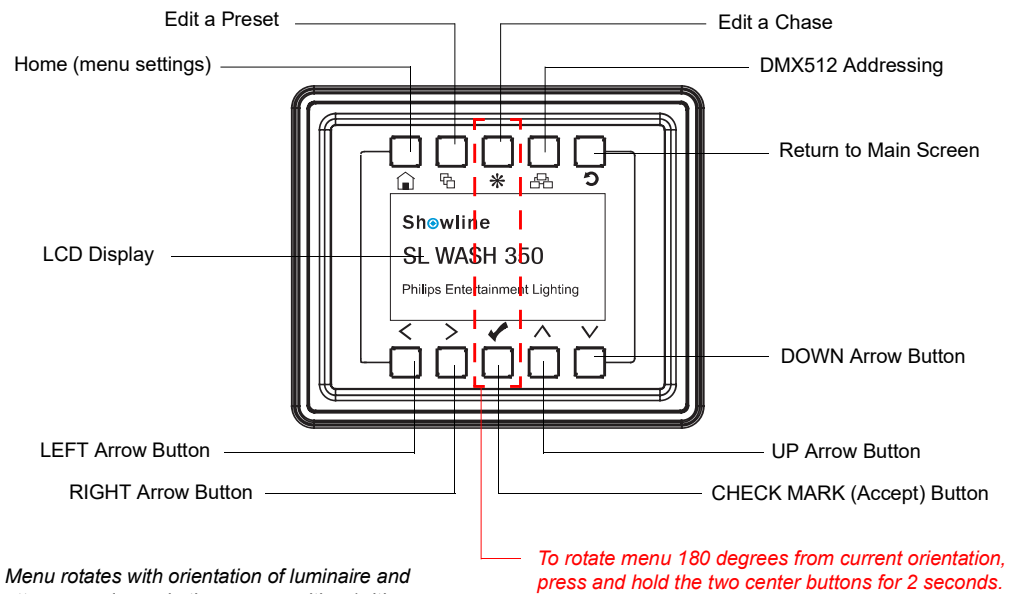
Figure 3: LCD Display & Menu System
