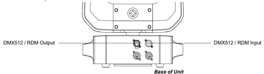
Figure 5: SL WASH 350 RGBW LED Luminaire DMX512 Input / Output Connections
