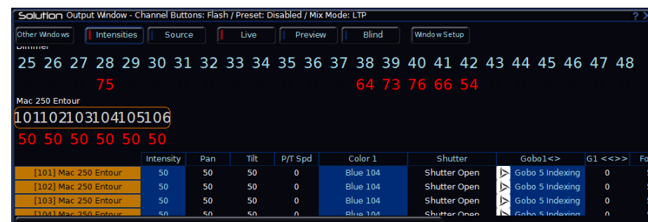
Figure 43 – Output Window showing Fixture Section
