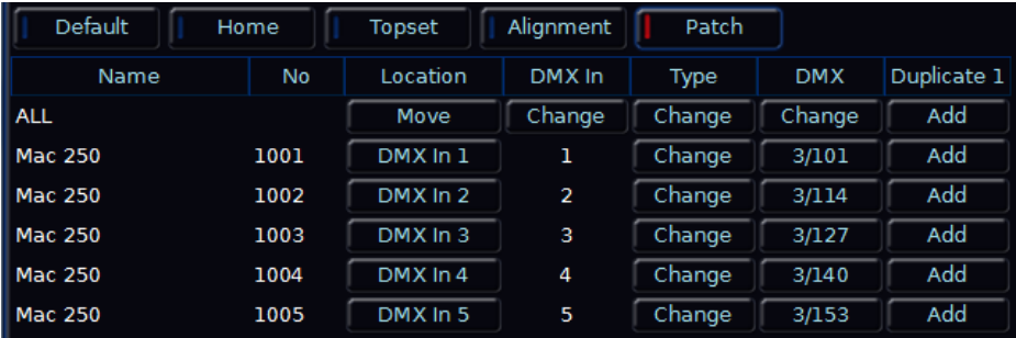
Figure 23 - DMX In Fixtures in Edit Fixtures
