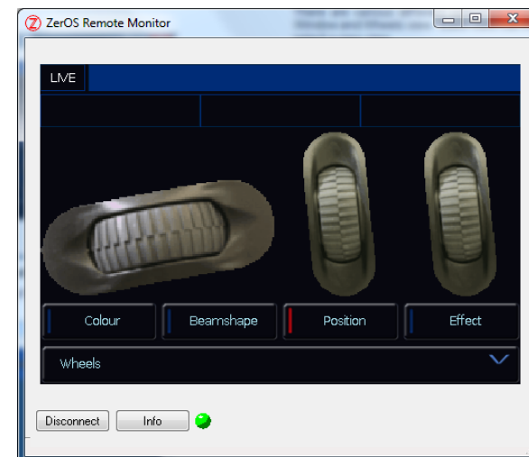
Figure 65 - Wheels Remote
