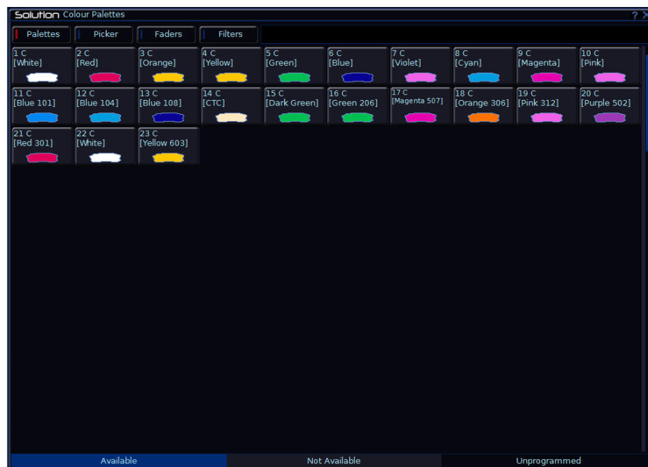
Figure 10 - Palette Window
