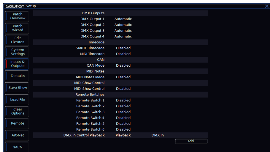
Figure 28 - Desk Setup
