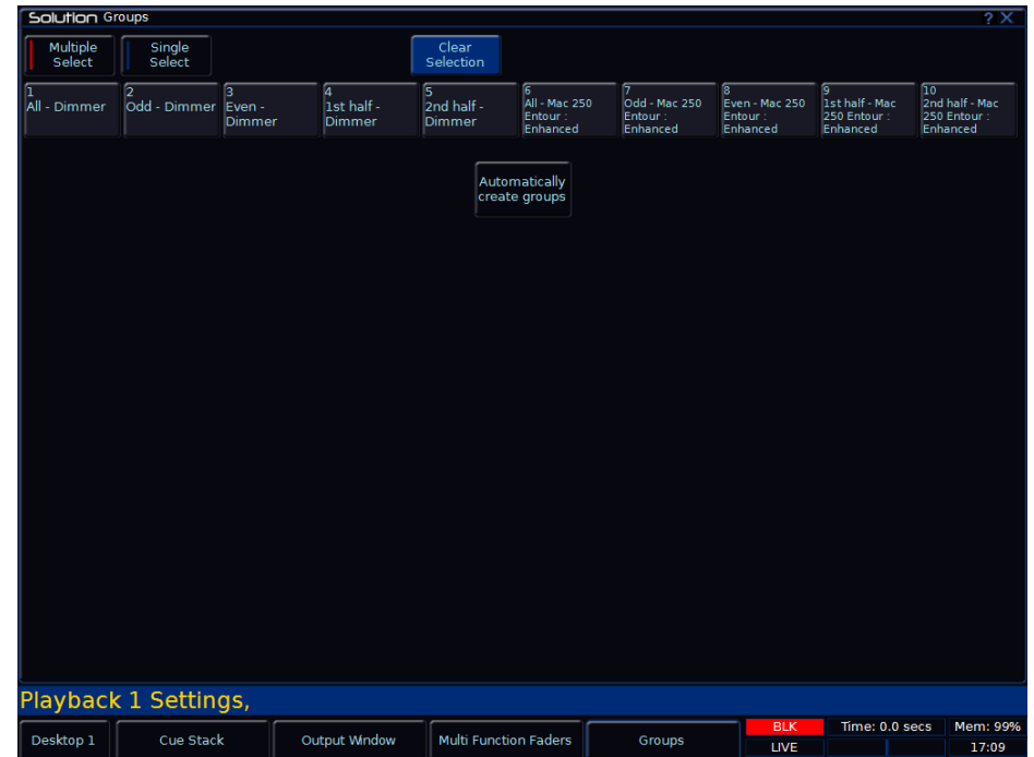
Figure 48 - Group Window
