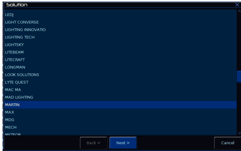
Figure 12 - Manufacturer Selection
