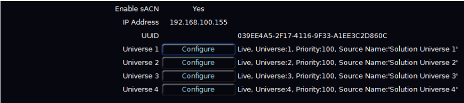
Figure 36 - sACN Configuration
