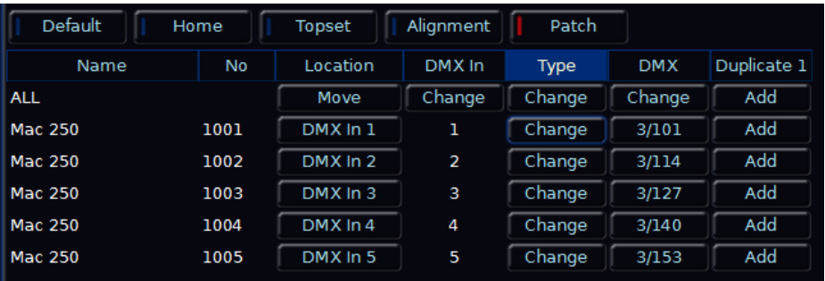
Figure 24 - Change Type
