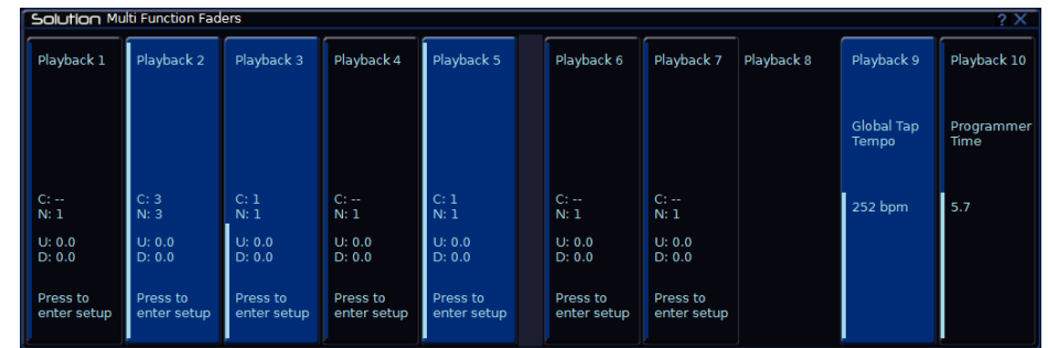
Figure 46 – MFF Window
