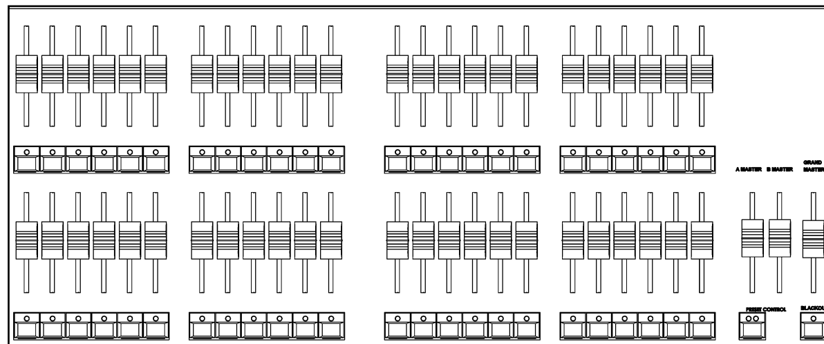
Figure 40 - Preset Faders
