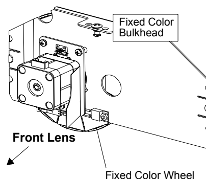
Figure 3-2: Fixed Color Bulkhead
