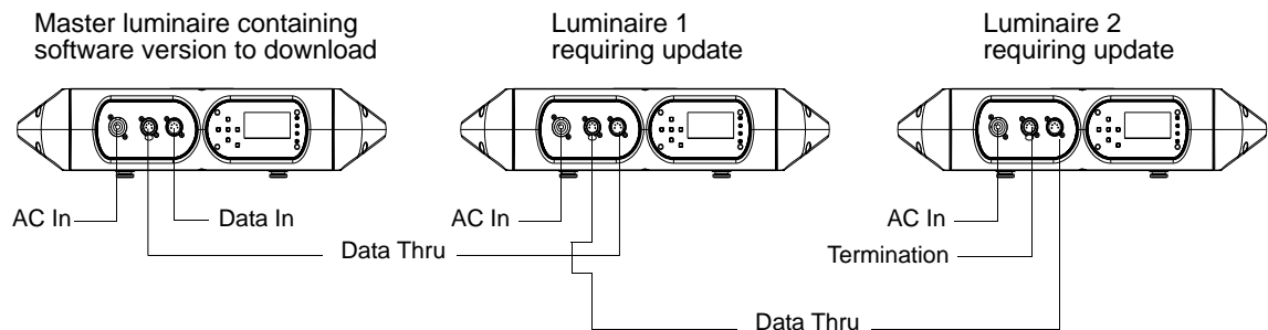
Figure 4-3: Test Setup
