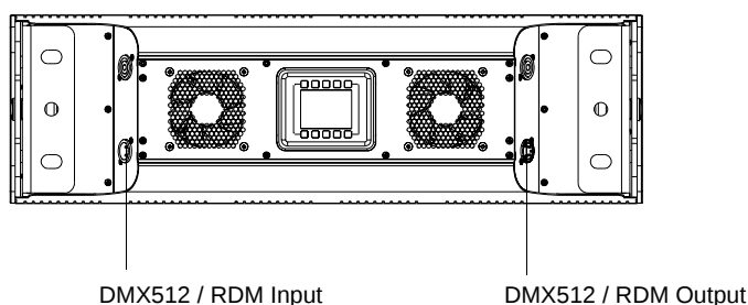
Figure 5: SL BAR 620 RGBW LED Luminaire DMX512 Input / Output Connections
