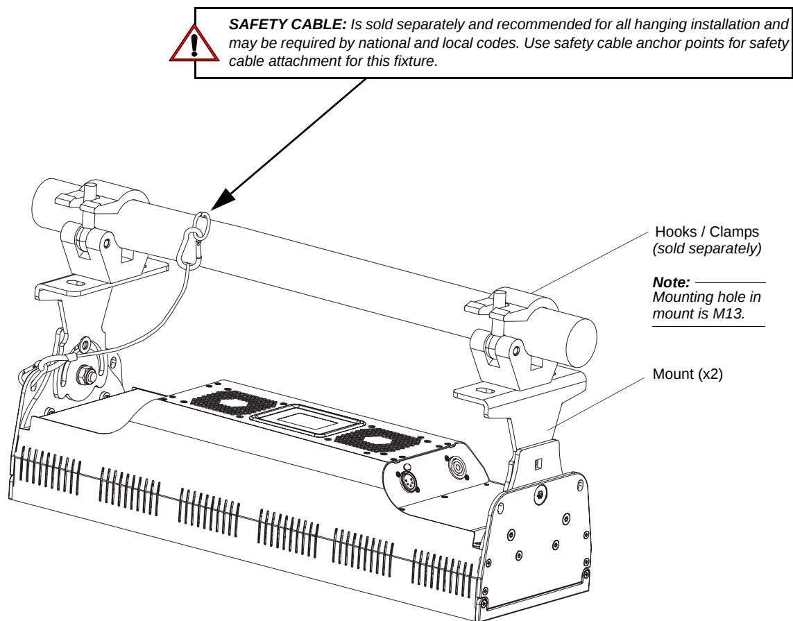
Figure 7: Mounting Luminaire
