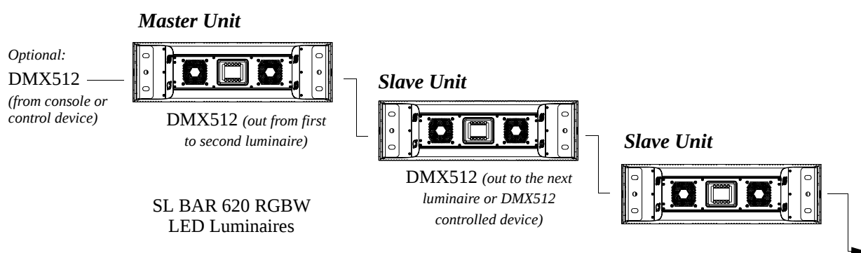
Figure 10: SL BAR 620 RGBW LED Luminaire - Master / Slave Configuration
