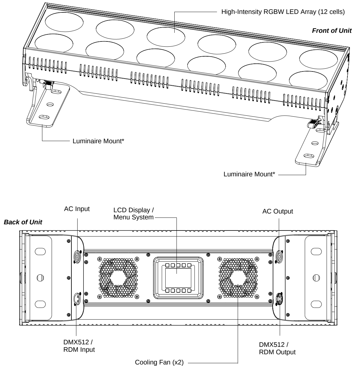
Figure 2: SL BAR 620 RGBW LED Luminaire Components
