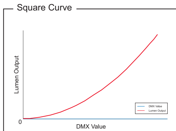
Figure 9: SL BAR 620 RGBW LED Luminaire Dimmer Curves
