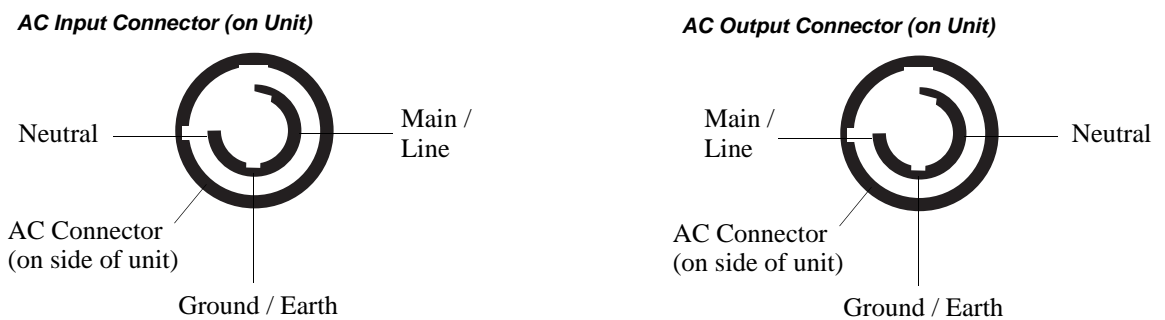
Figure 4: SL BAR 660 RGBW LED Luminaire AC Input & Output Connections
