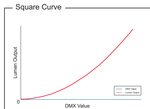
Figure 9: SL BAR 660 RGBW LED Luminaire Dimmer Curves
