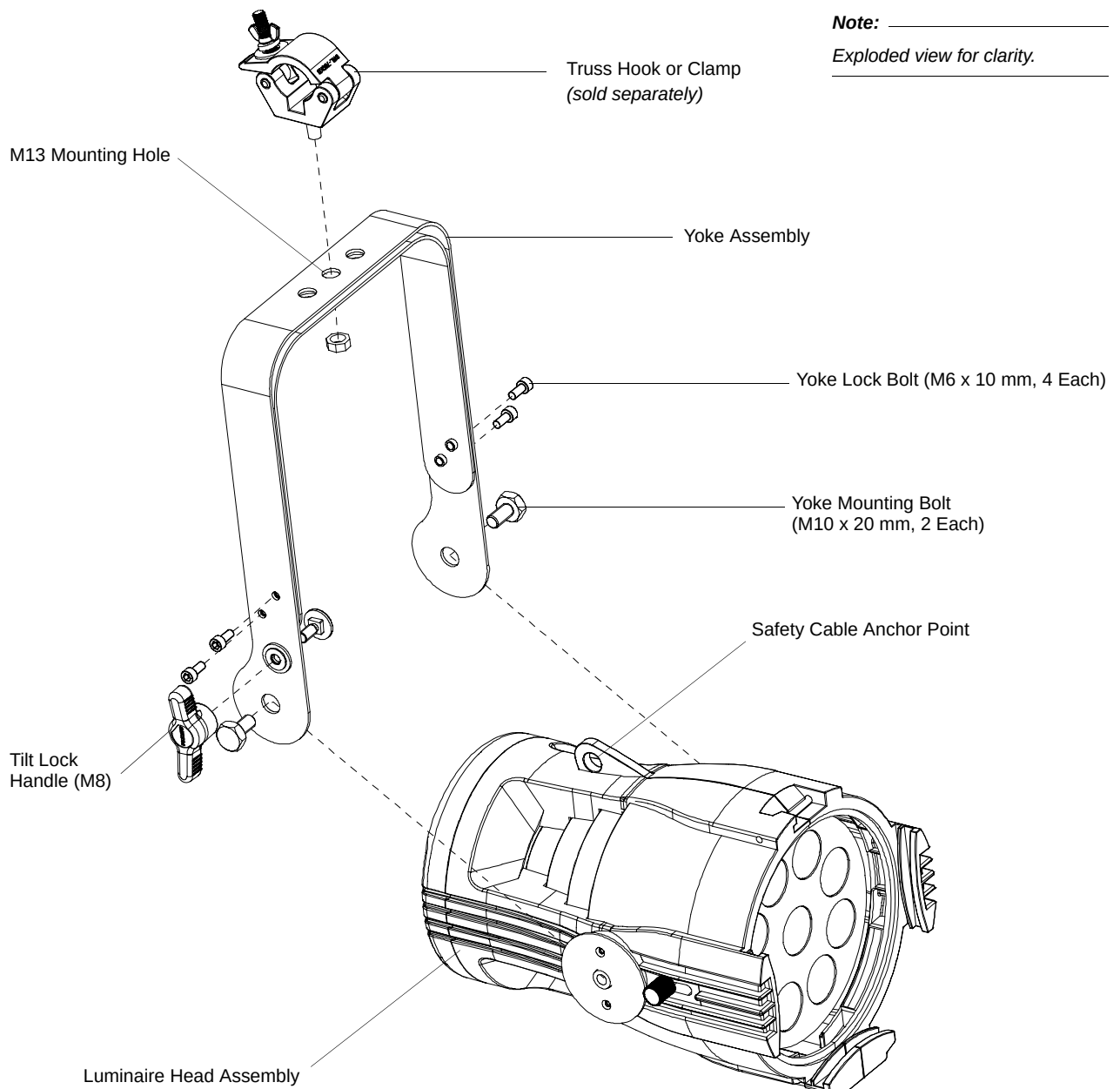
Figure 7: Luminaire and Yoke Components
