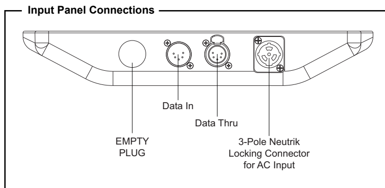
Figure 2: Power Connector
