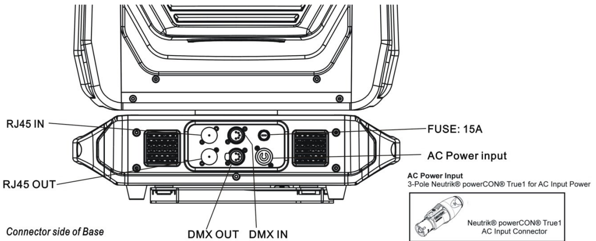
Figure 2: Power Connector
