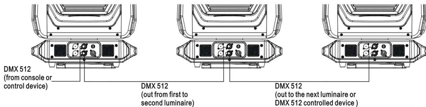
Figure 3: Data Link
