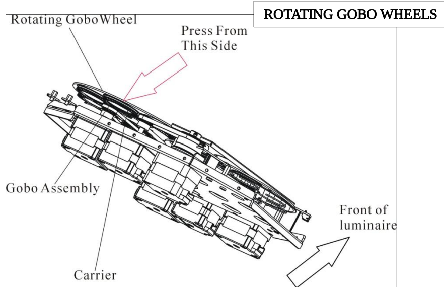
Figure A-3: Replacing Gobos
