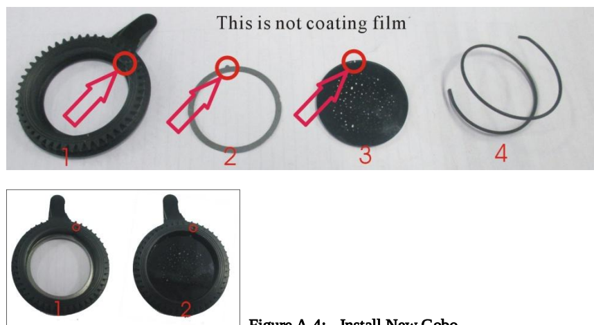
Figure A-4: Install New Gobo
